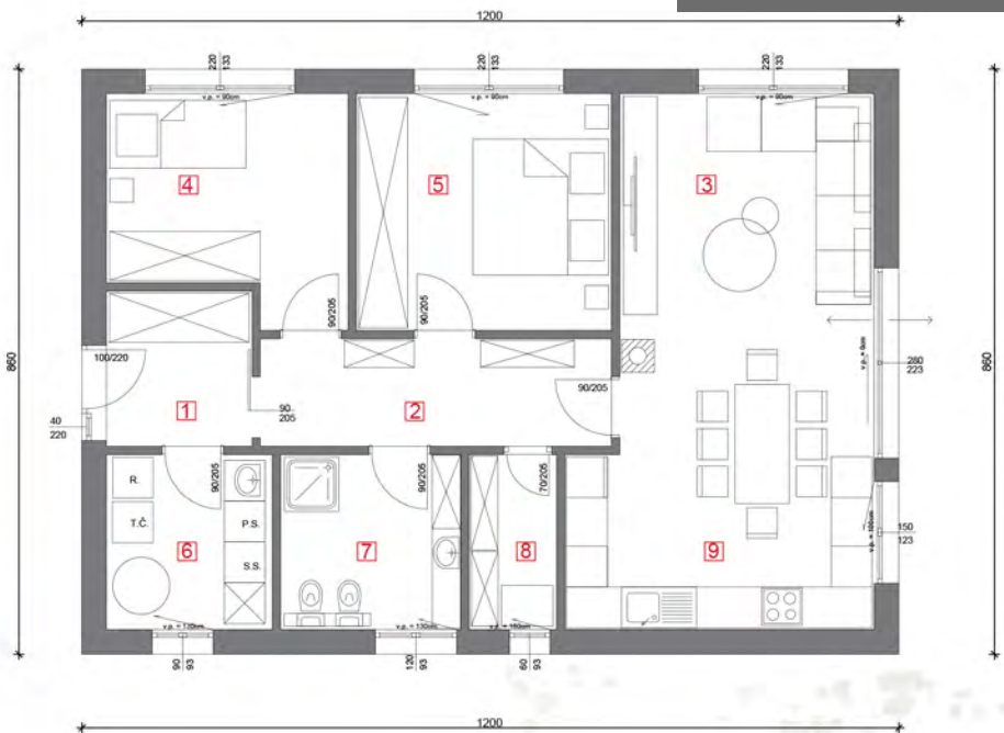
MK TIP Grita
